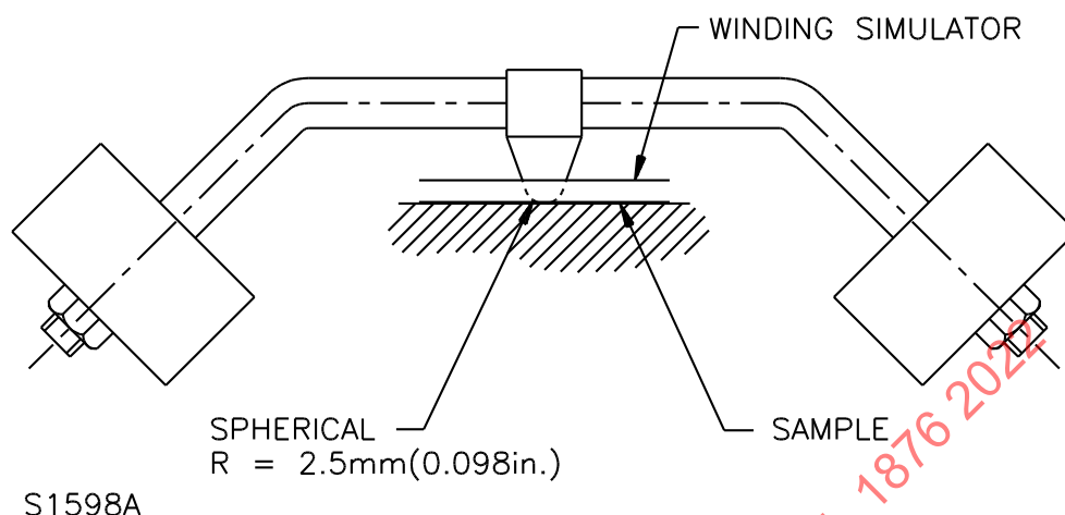
Figure 20.2 Ball-pressure apparatus
