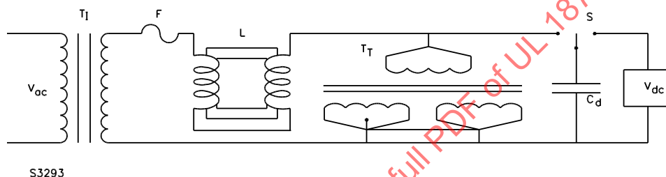
Figure 21.1 Circuit for voltage surge
