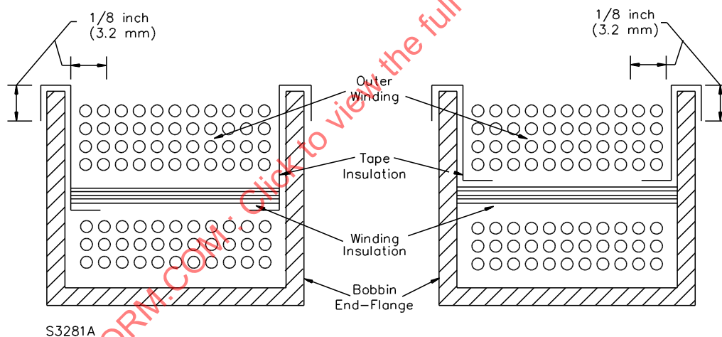
Figure 12.3 Bobbin wound transformer with overlapped tape
