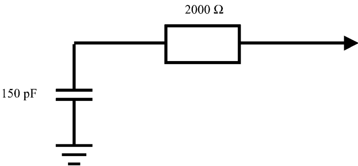
FIGURE 1B—PACKAGING AND HANDLING TEST SIMULATOR PARAMETERS
