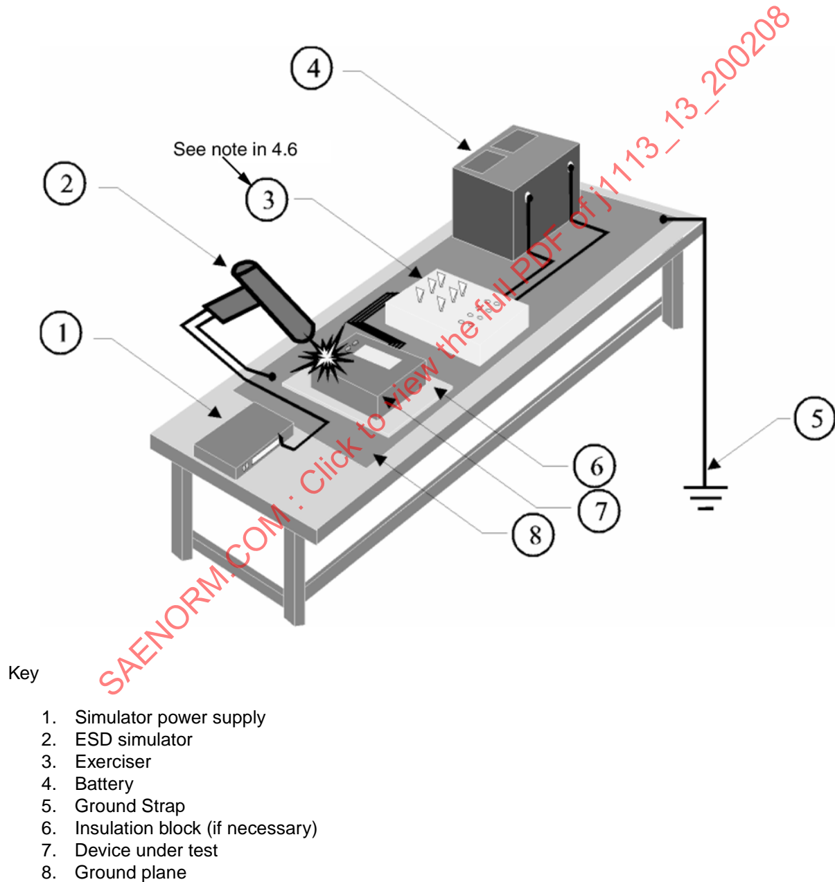
FIGURE 3—TEST SETUP FOR POWERED MODE COMPONENT TEST
