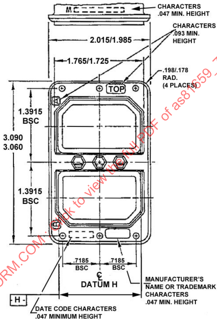
FIGURE 1 - CONNECTOR CONFIGURATION AND DIMENSIONS
