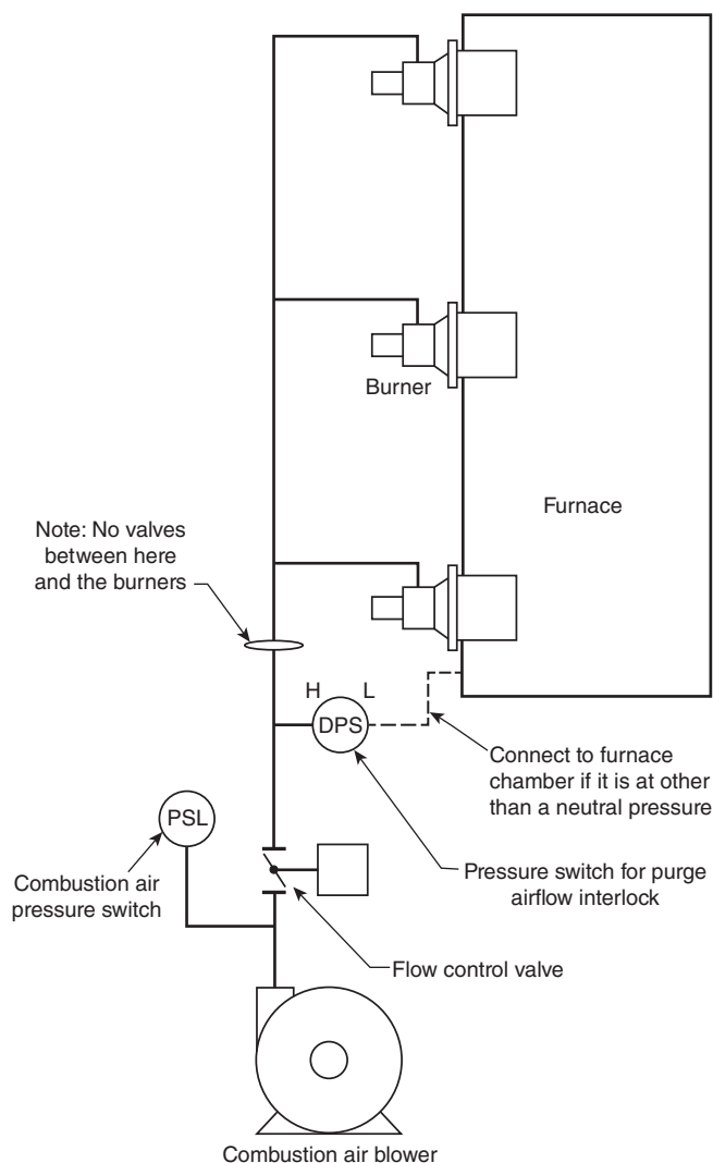
N FIGURE A.8.4.1.2.6 Example of Use of a Pressure Switch for Purge Airflow Interlock.
