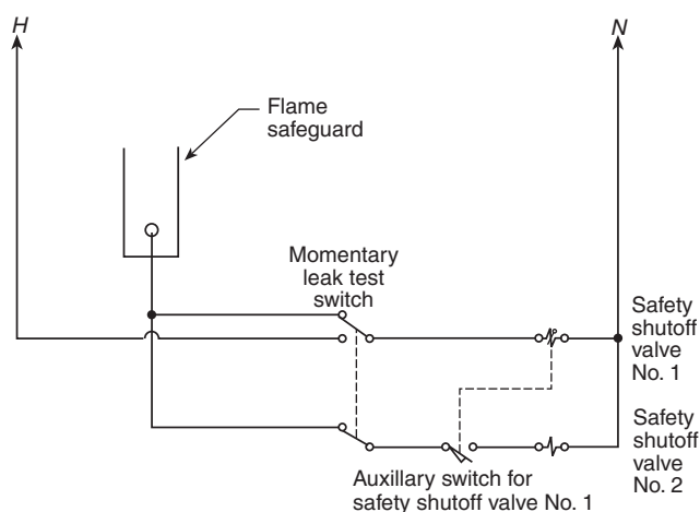
FIGURE A.7.4.10(b) Example of a Wiring Diagram for Leak Test.
