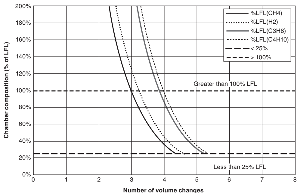
FIGURE A.8.4.1.2.1 Number of Perfectly Stirred Purge Volumes to Reach 25 Percent LFL (Starting with 100 Percent Fuel).
