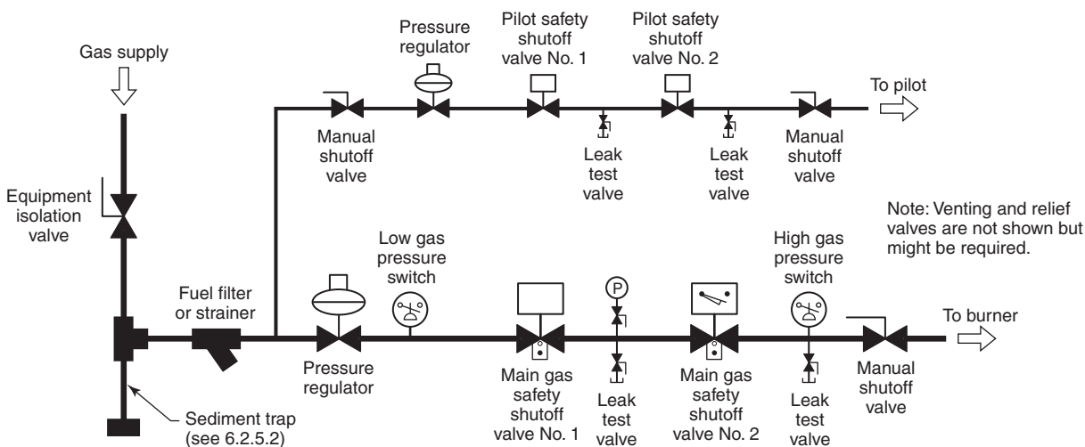
FIGURE A.8.7.2.3 One Example of a Leak Testing Arrangement.
