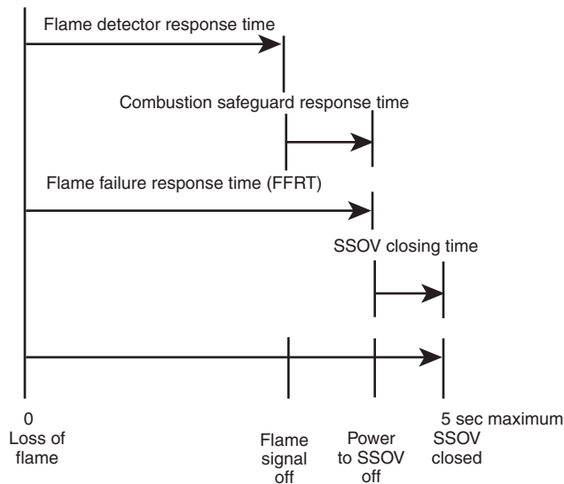
FIGURE A.8.9.3 Response Times on Loss of Flame.
