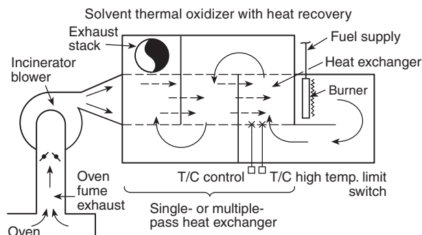
FIGURE A.10.6.3 Example of a Thermal Oxidizer System with Recuperative-Style Heat Recovery.
