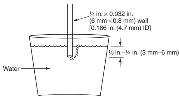
FIGURE A.7.4.10(c) Leak Test for a Safety Shutoff Valve.
