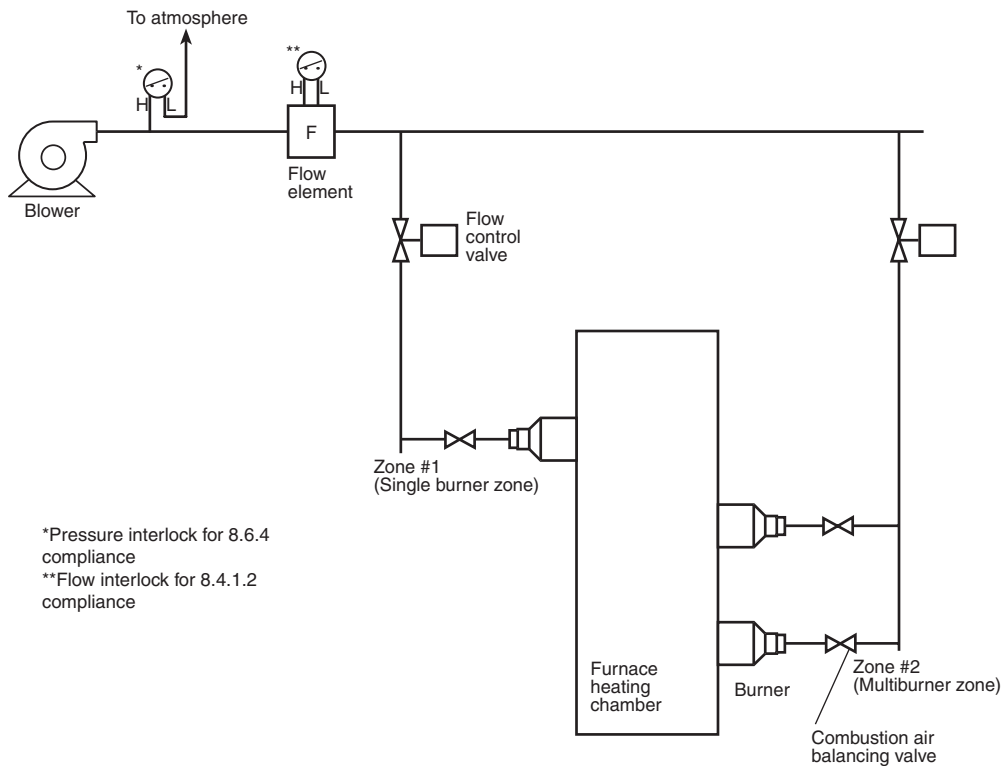
FIGURE A.8.6.4 Examples of Air Proving Devices Used in Multiburner Systems (fuel piping not shown for clarity).
