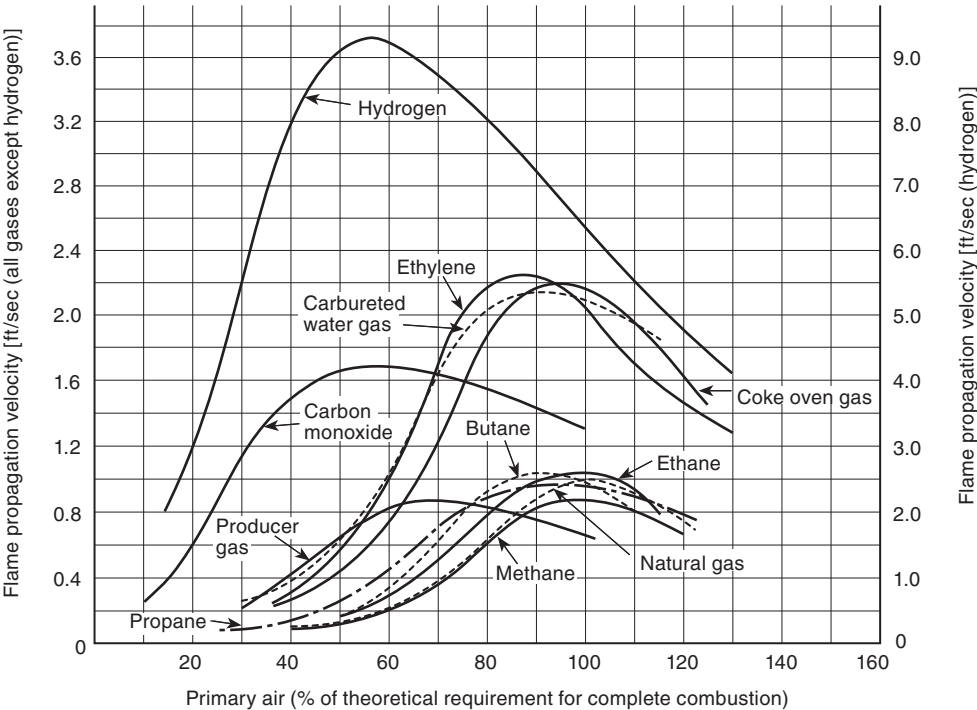
Δ FIGURE A.6.2 Ignition Velocity Curves for Typical Flammable Gases.
