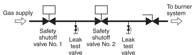
FIGURE A.7.4.10(a) Example of a Gas Piping Diagram for Leak Test.
