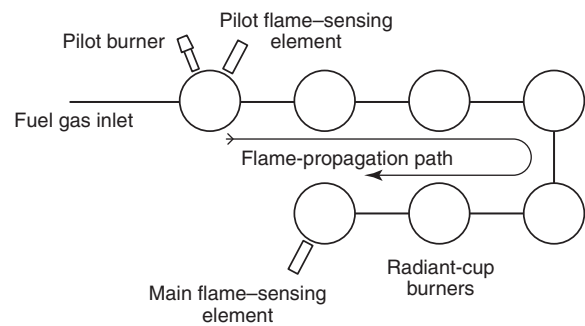
FIGURE A.8.9.6(b) Example of a Combustion Safeguard Supervising a Group of Radiant Cup Burners Having Reliable Flame-Propagation Characteristics from One to the Other by Means of Flame-Propagation Devices.
