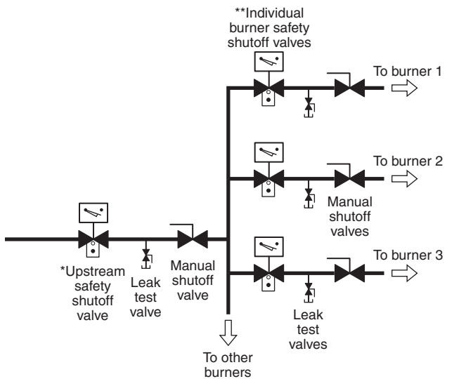
FIGURE A.8.7.1.12 Multiple Burner System Using Proof-of-Closure Switches.
