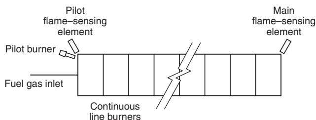
FIGURE A.8.9.6(a) Example of a Combustion Safeguard Supervising a Pilot for a Continuous Line Burner During Light-Off and the Main Flame Alone During Firing.
