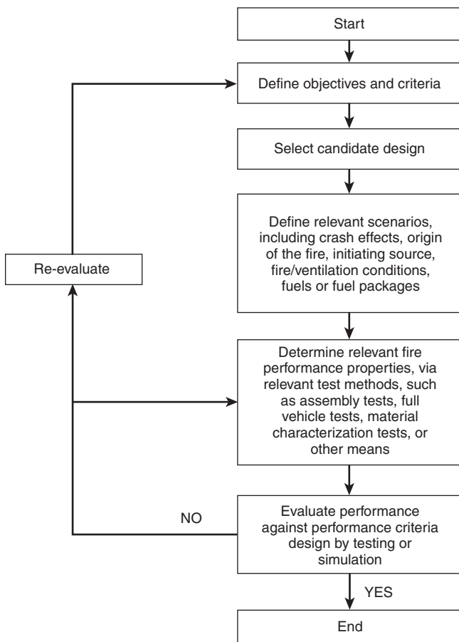
FIGURE 6.2.1 Flow Chart for the Performance-Based Approach to Be Used in This Guide.
