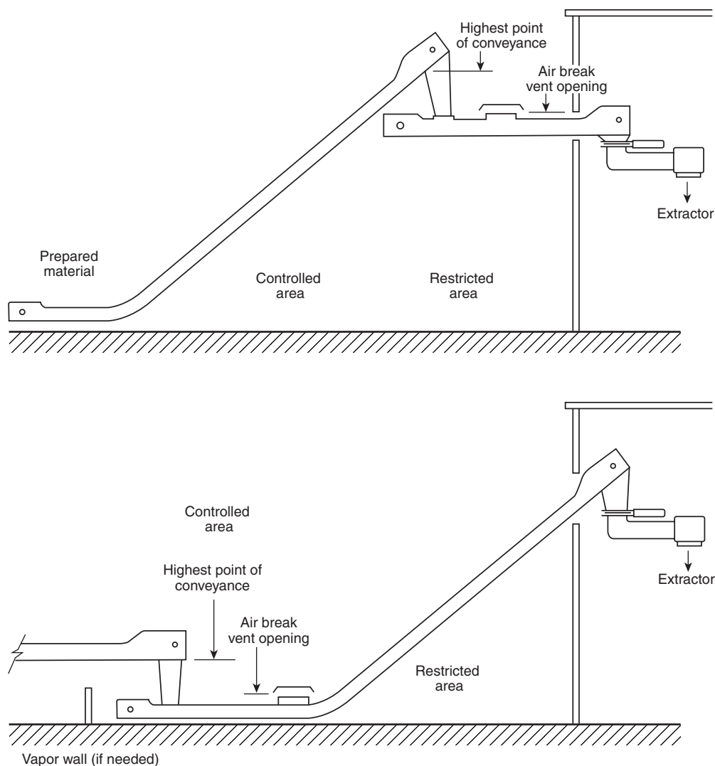
FIGURE 7.5.2 Typical Locations for Air Break Vent Opening.
