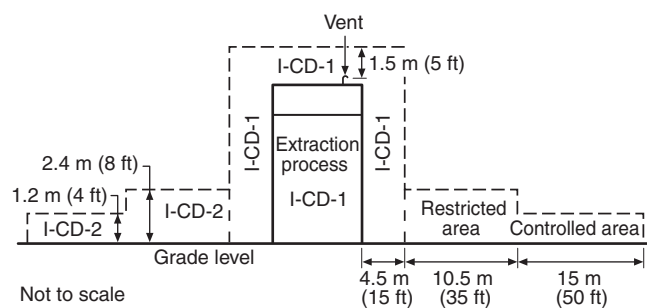
FIGURE 7.7.1 Type and Extent of Hazardous Areas.
