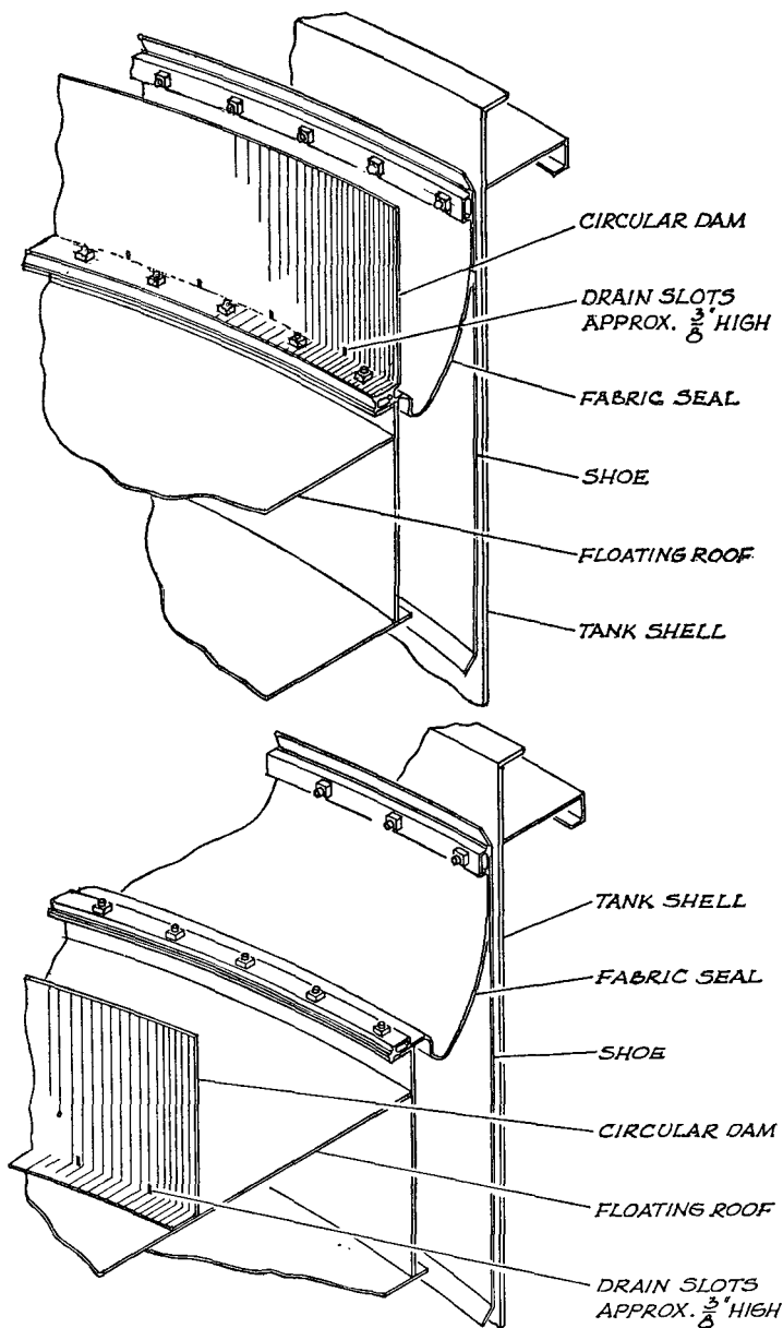
Fig. A-3311. Typical Foam Dams for Floating Roof Tank Fixed Protection.
