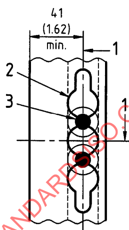
View B
