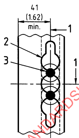
View B
