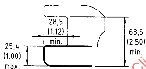
Section A-A Typ. 4 edges
