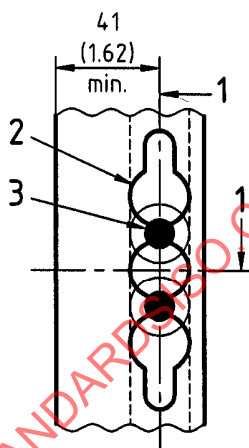
View B
