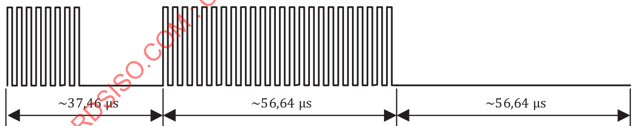
Figure 16 — End of frame when using one subcarrier
