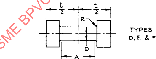
FIG. 2 Alternative Tension Test Specimens
