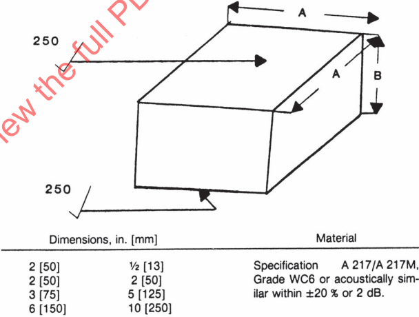
FIG. 3 CALIBRATION BLOCKS
